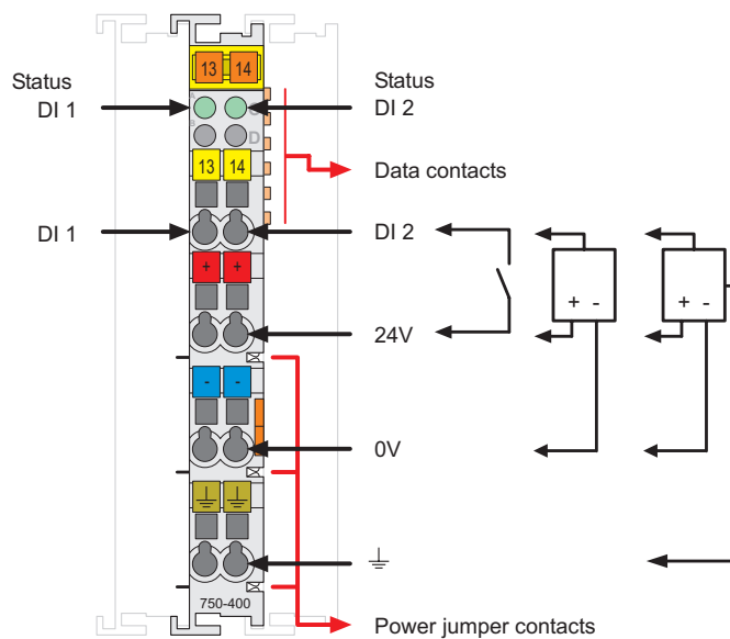
Fig. 2.1.1-1: 2-Channel Digital Input Module 750-400
