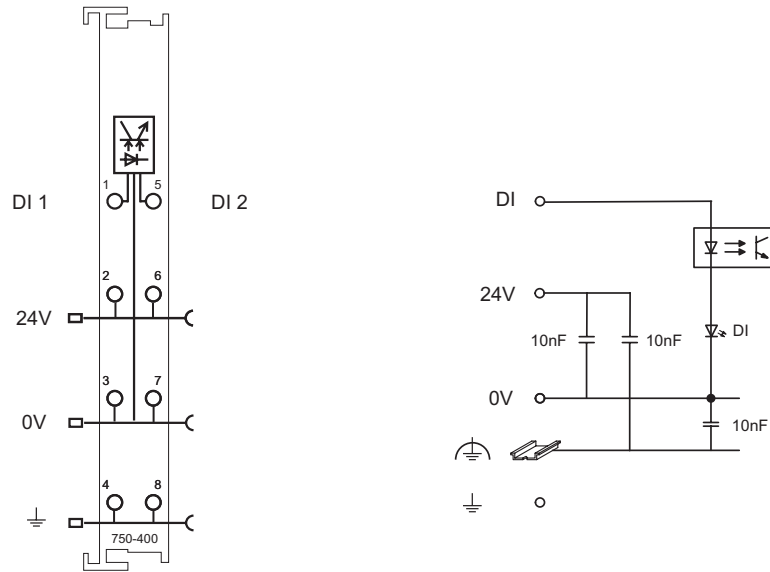
Fig. 2.1.1-3: 2-Channel Digital Input Module 750-400
